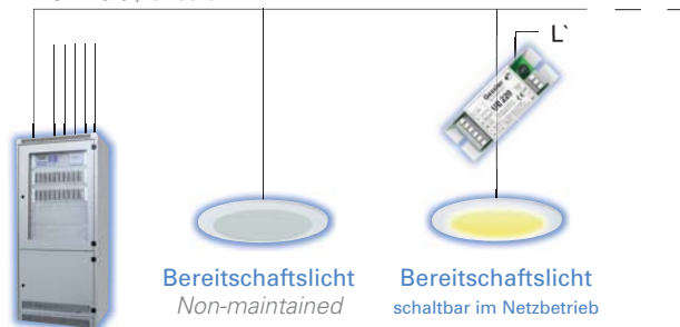
BS-Kreis / circuit
